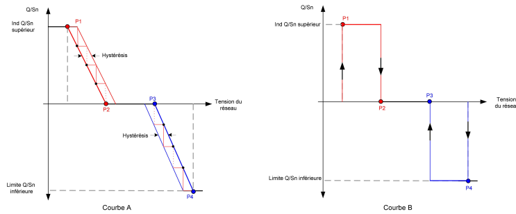
Figure 7-19 Courbe Q(U)
