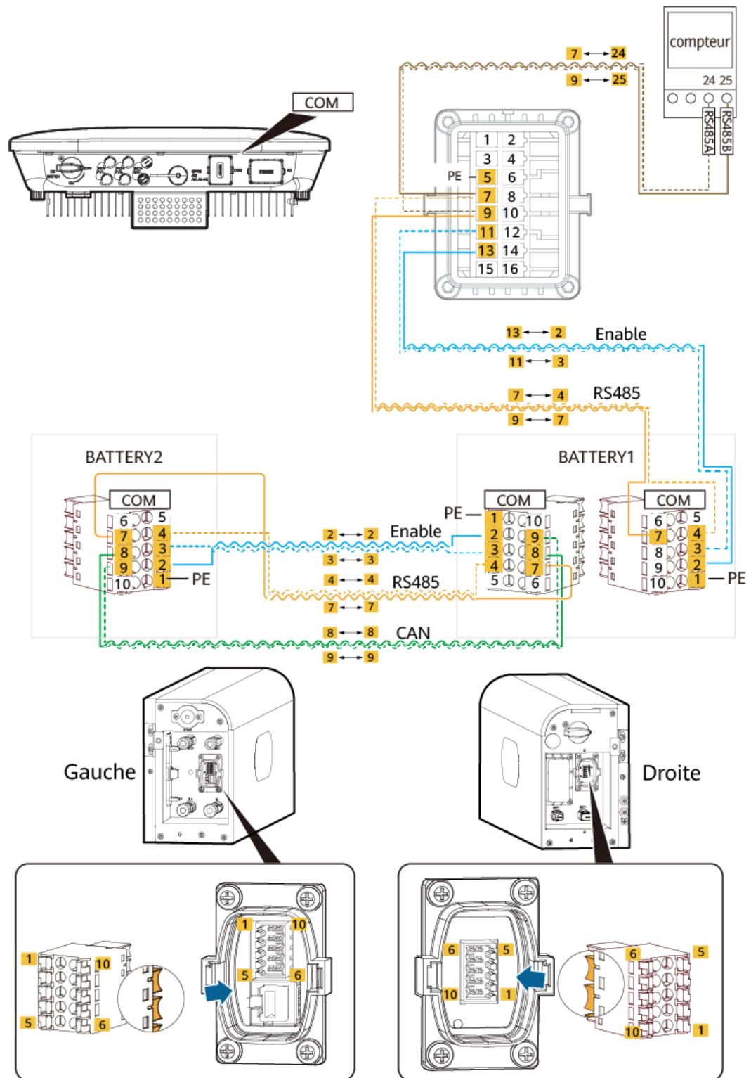
Figure 6-7 SUN2000-(3KTL-12KTL)-M1
