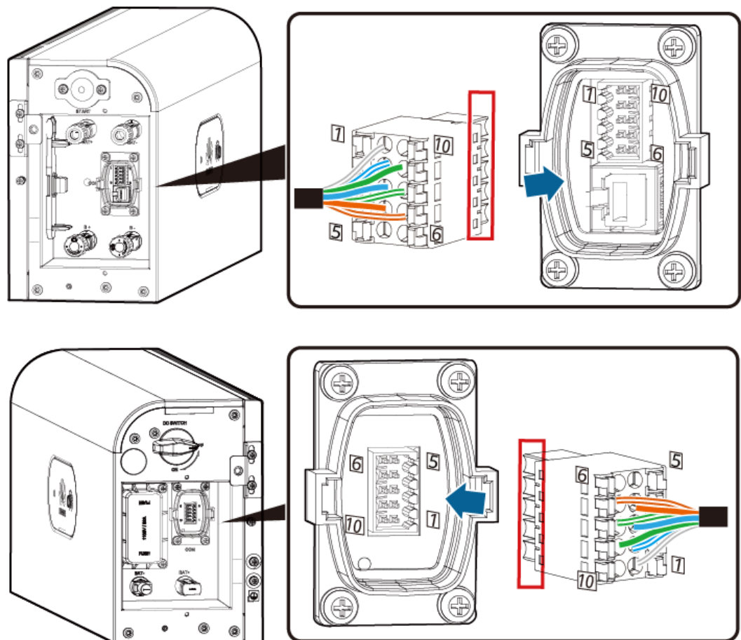
Figure 6-17 Insertion de la borne
