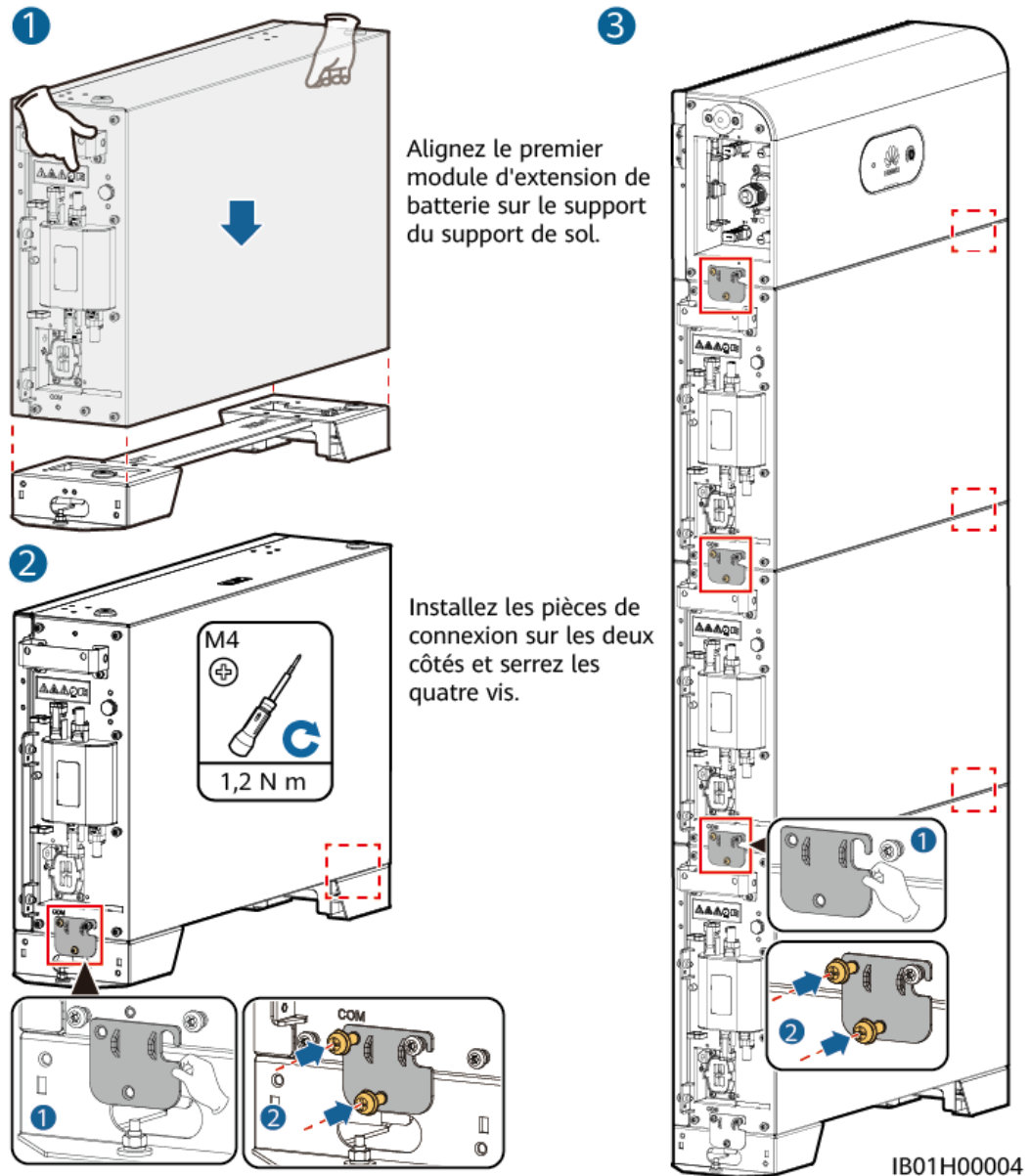
Figure 5-8 Installation murale
